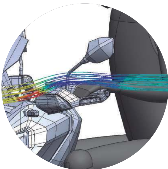
ORIGINAL HANDGUARD
