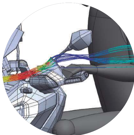
HANDGUARD EXTENSION
