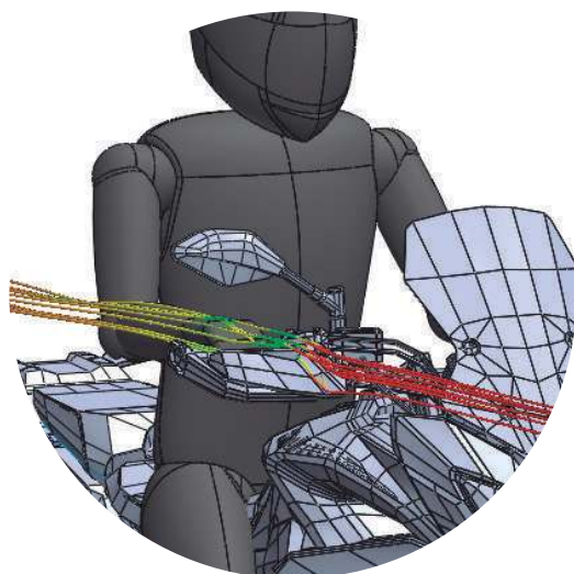
ORIGINAL HANDGUARD
